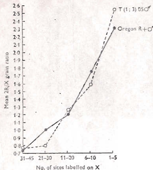
Text-fig. 2. Mean 2R/X 3 H-TdR grain ratio in different labelling patterns of the male X in normal and insertion stock.
