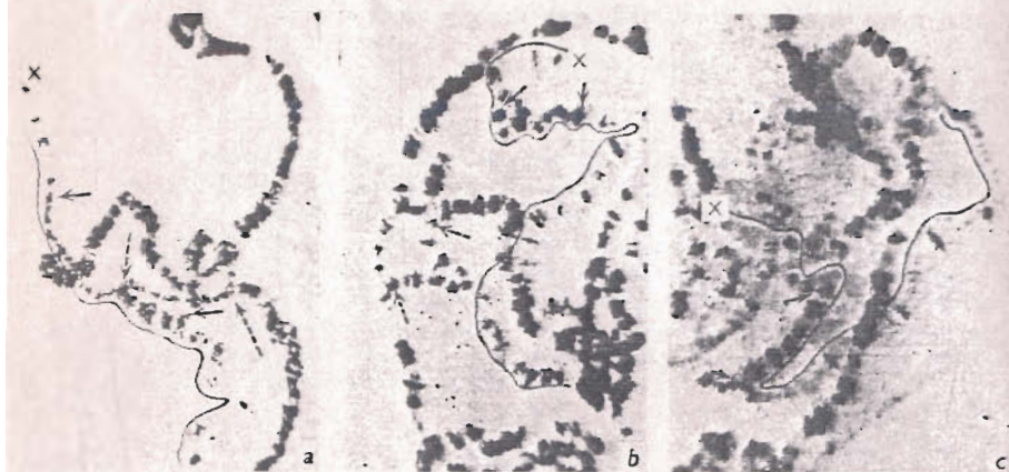
Plate 2. ^3\text{H-TdR} labelling patterns in salivary gland chromosomes of T(1;3)05 male larvae. Solid line indicates the orientation of the X; solid arrows the inserted autosomal segment and broken arrows the non-translocated homolog of the insertion in unpaired condition. (a) Autosomes and the insertion are continuously labelled, the X shows discontinuous label. The insertion is partly paired with its homolog. (b) and (c) Autosomes and the insertion showing discontinuous label, while the X shows label at still fewer sites. In (b) the inserted segment is completely unpaired, in (c) completely paired. Note the similarity of labelling patterns in the inserted segment and its homolog.
