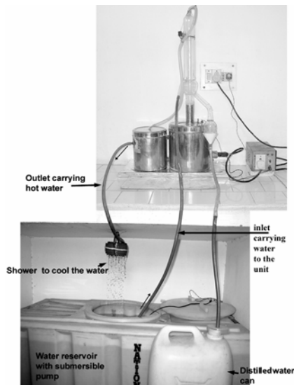
Figure 1. Distillation plant assembly.
